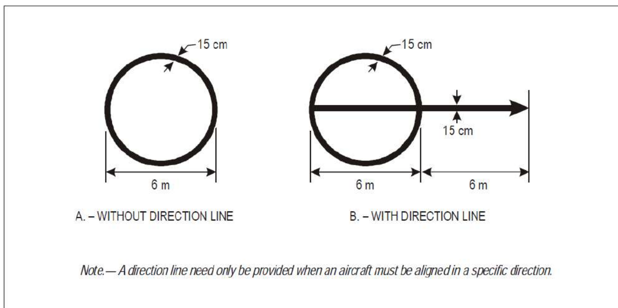
Figure H-9. VOR Aerodrome checkpoint marking.
