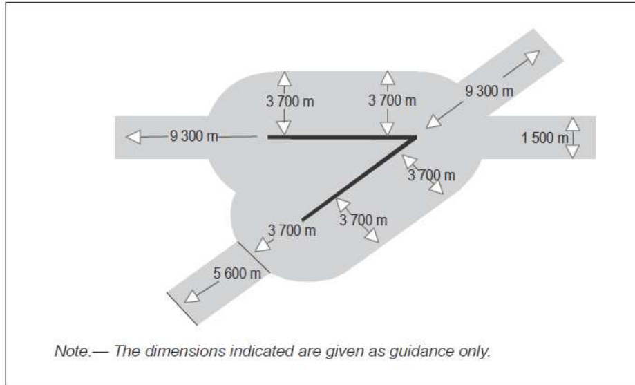
Figure H-12. Multiple runway laser-beam flight zone
